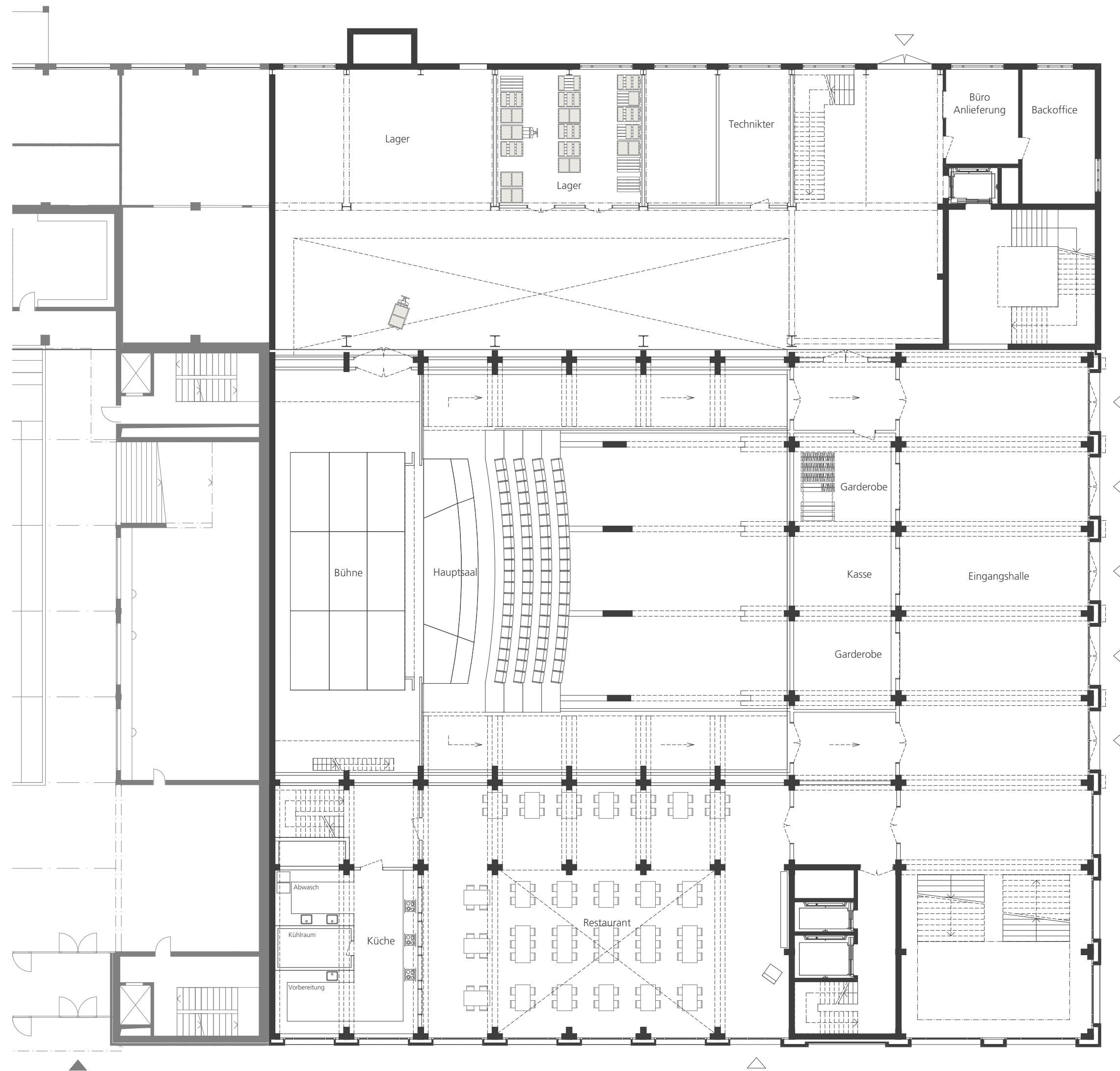
Erdgeschoss | 1:200
