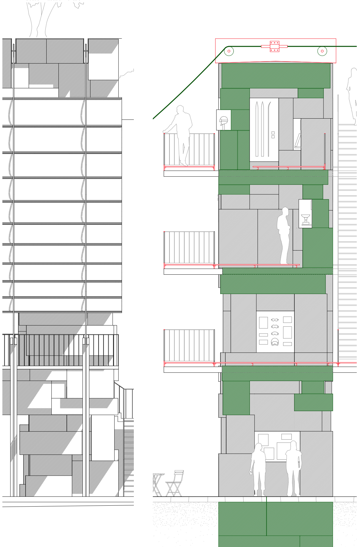
ABB. 117 Section Facade/Elevation
