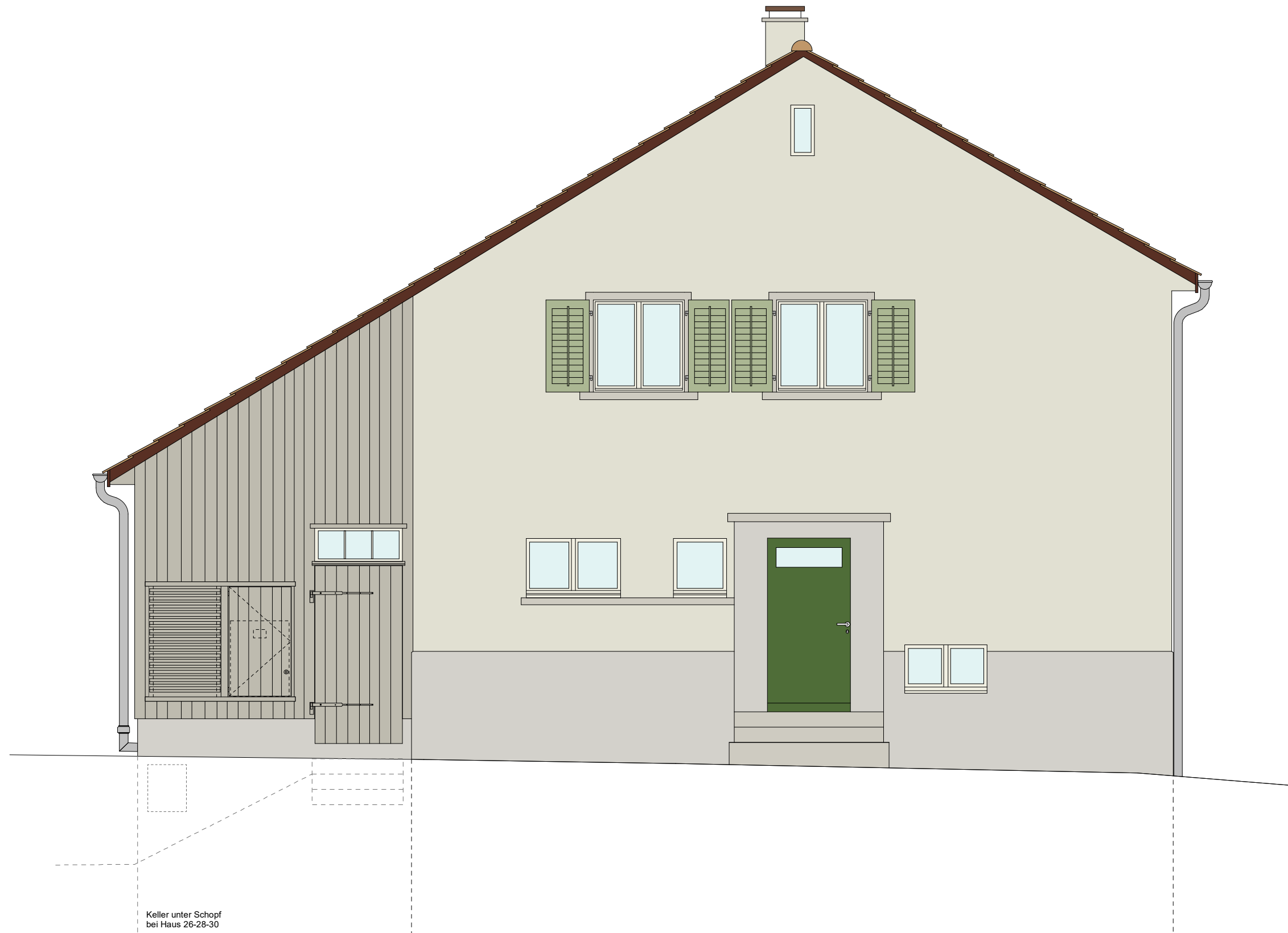
Fassade West
