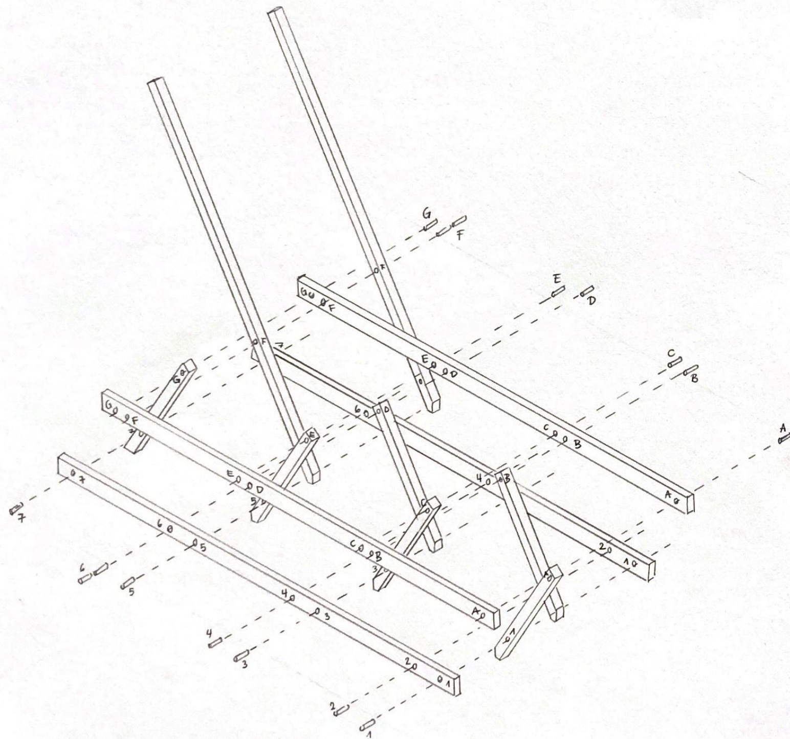
CONSTRUCTION OF SINGLE ELEMENT
