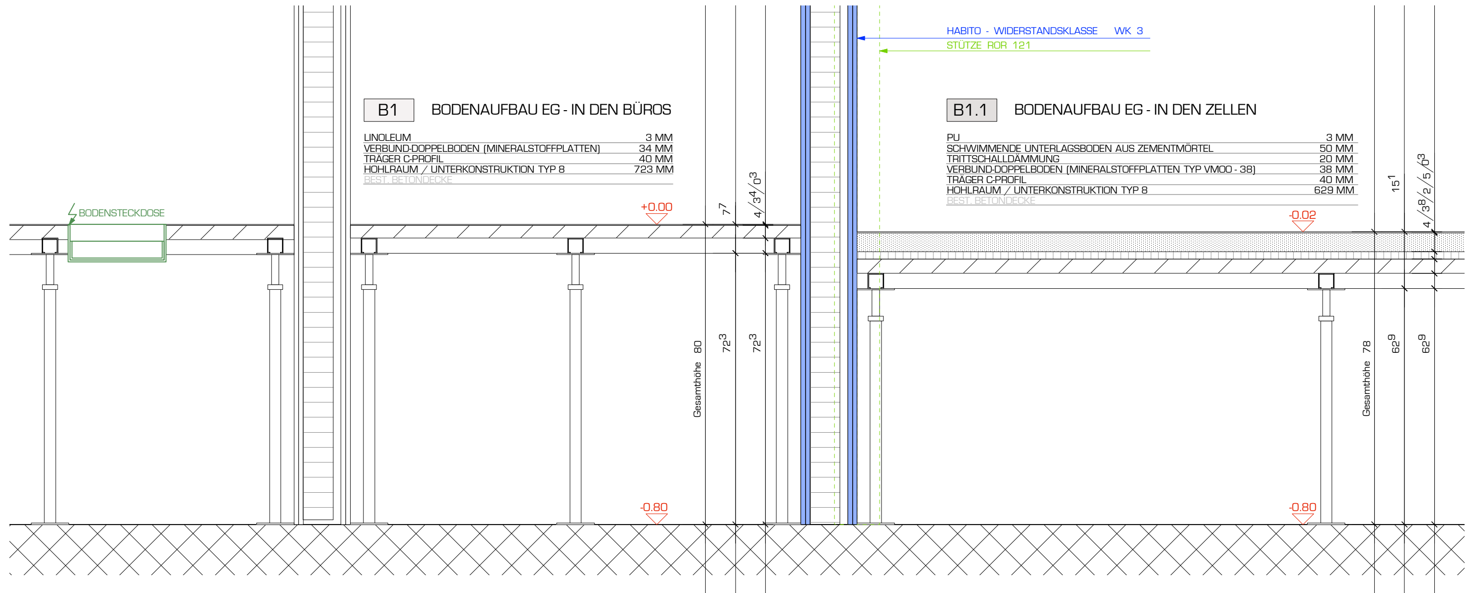
DETAIL 2 1/10
