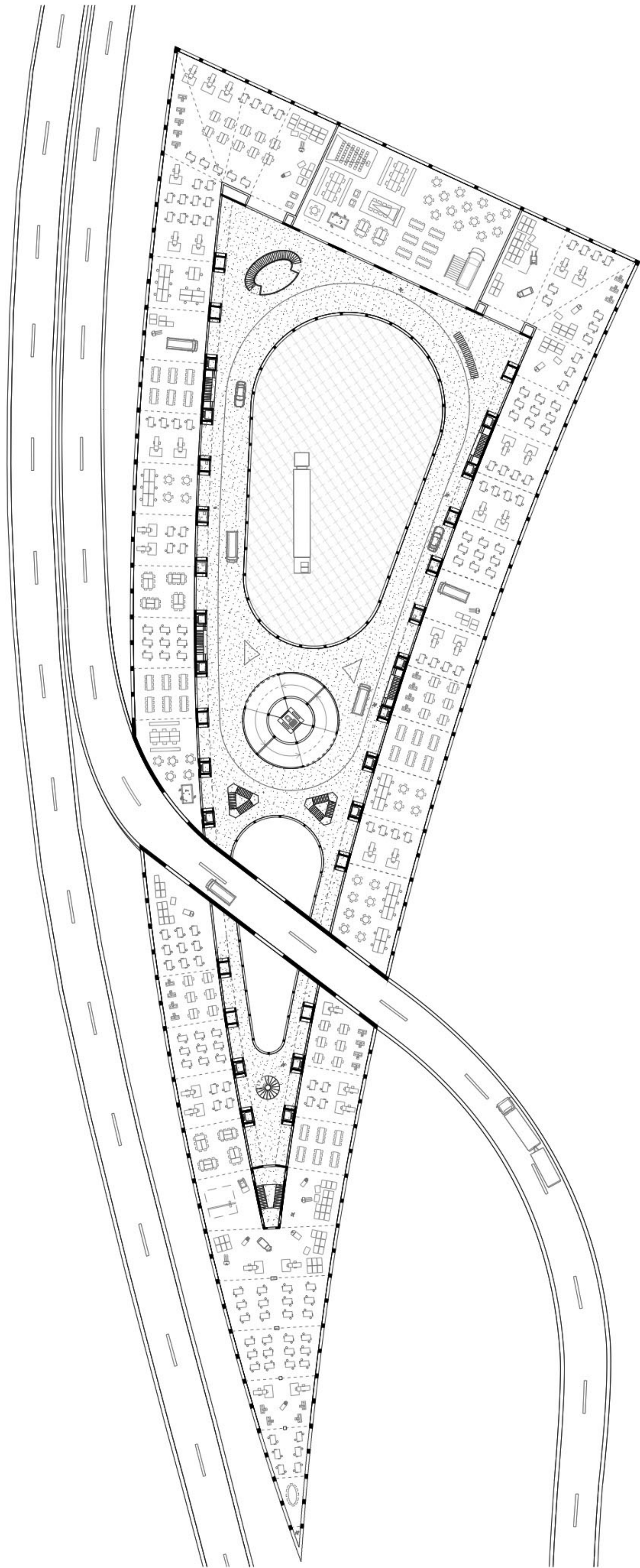
1st Floor - Workshops, Great Hall, Highway breaking through the building 1:500
