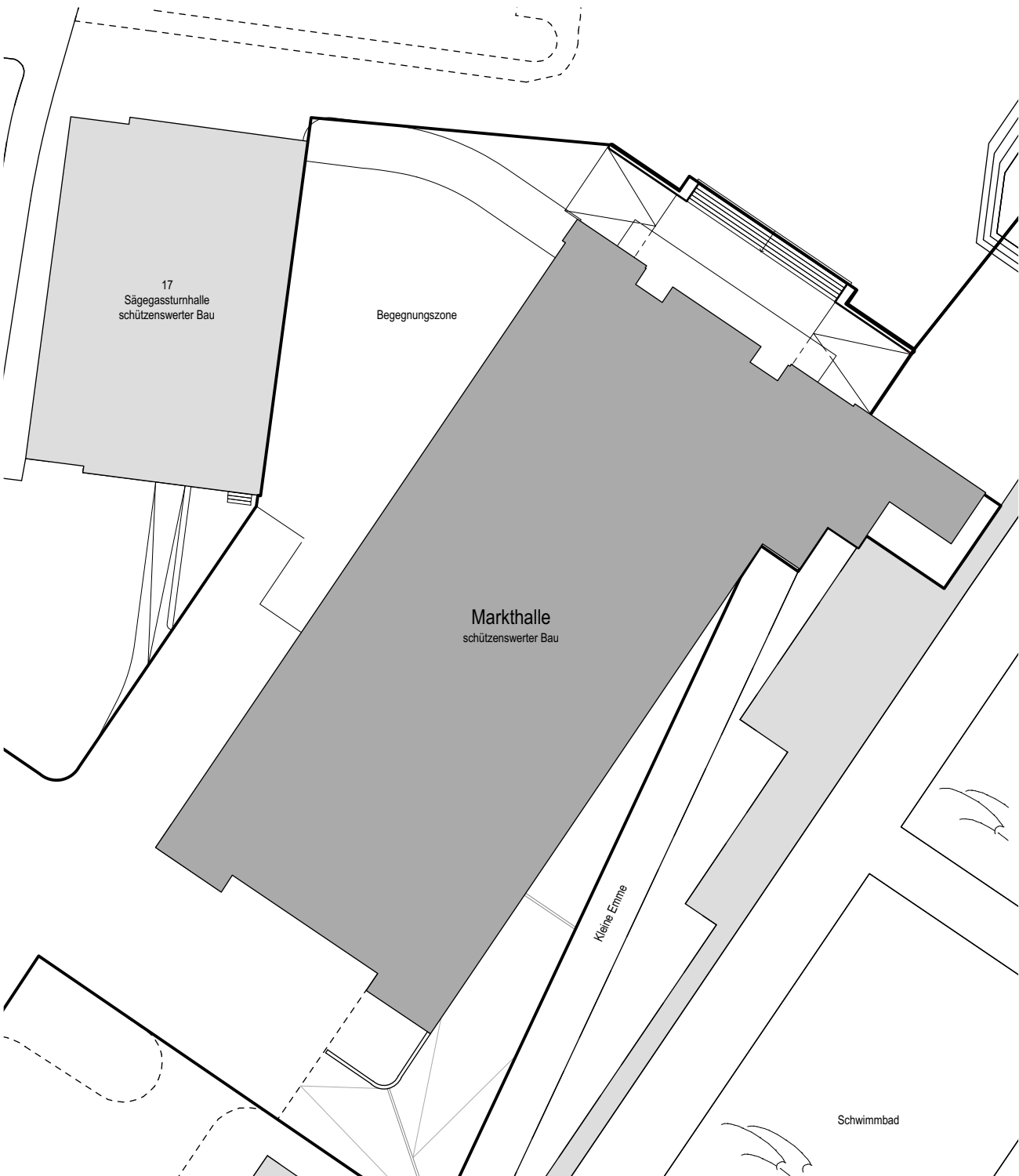
Situation 1:500
