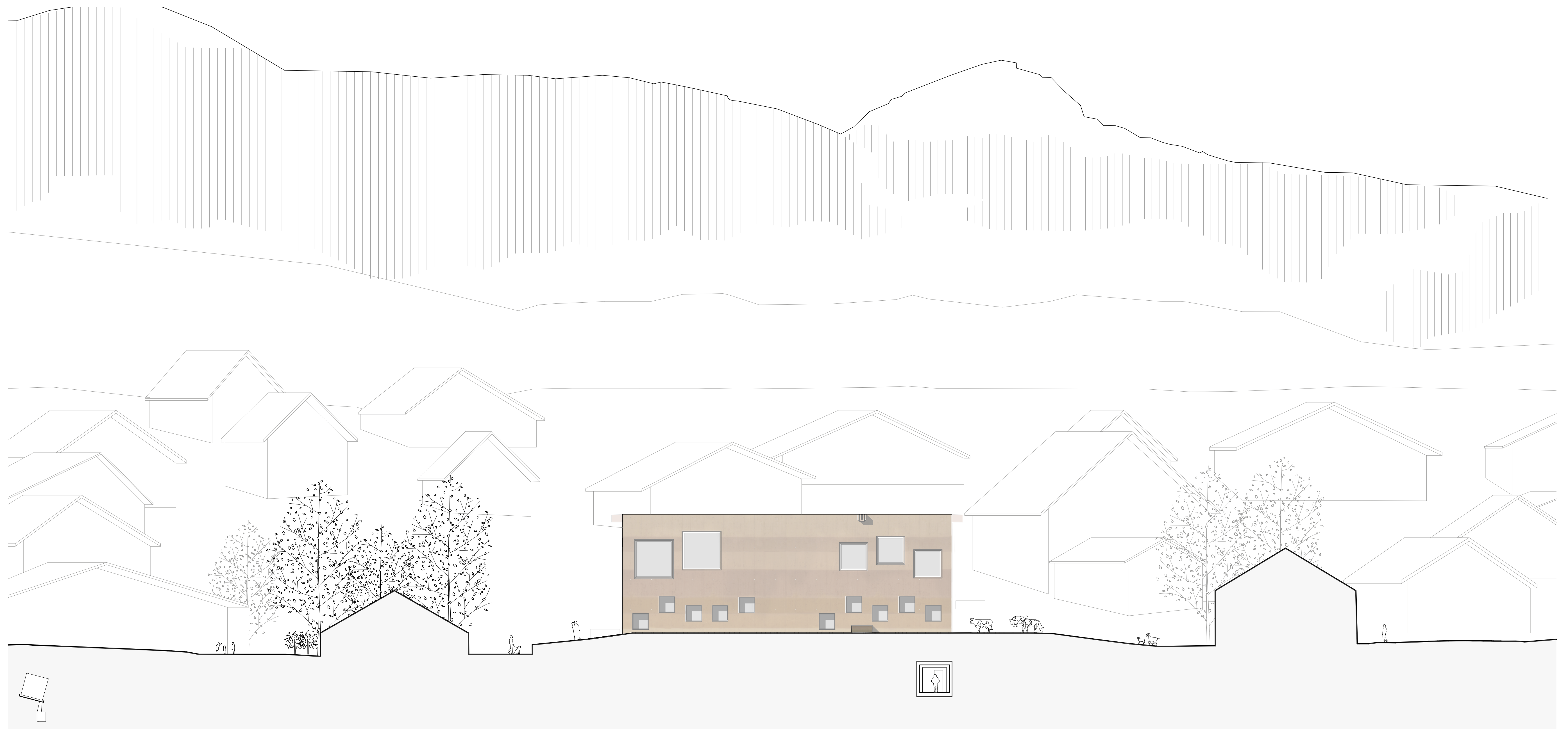
ELEVATION FACADE SUD 1:200
