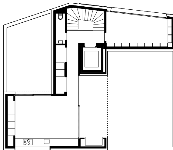
Attikageschoss 1:200
