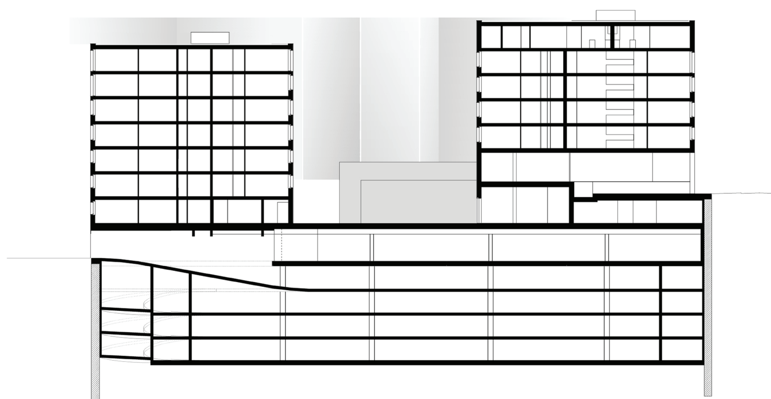
Coupe E-O
